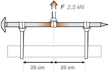
Pull Test
