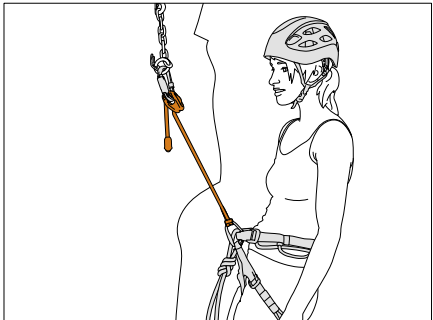
The CONNECT ADJUST single lanyard allows the user to tether to the anchor when climbing or mountaineering in order to manage rope or gear, such as setting up a top rope or getting ready to belay.
