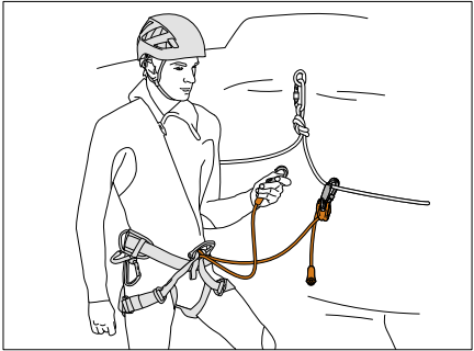
The DUAL CANYON CLUB and DUAL CANYON GUIDE lanyards allow positioning at the anchor and progression along a lifeline when canyoning.
