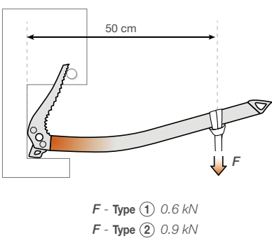
Shaft Insertion Strength Test
