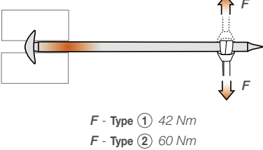
Levering Test
