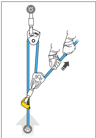
Pulley System
