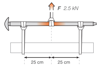
Pull Test
