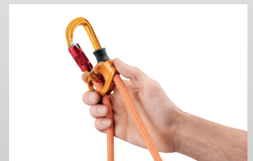
Smooth and precise length adjustment due to the ergonomic shape of the ADJUST rope adjuster.
